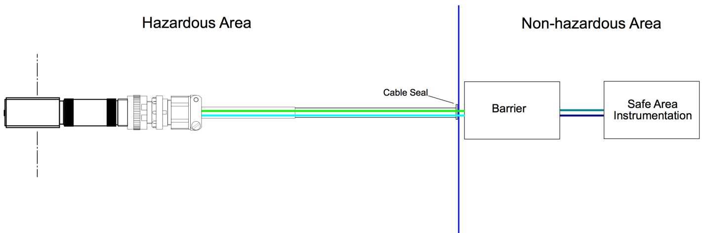
Figure 1: Typical connection arrangements
